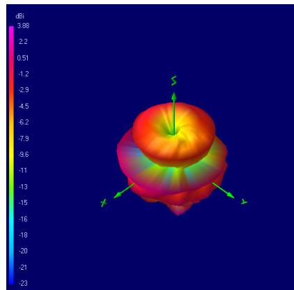
5544 MHz
