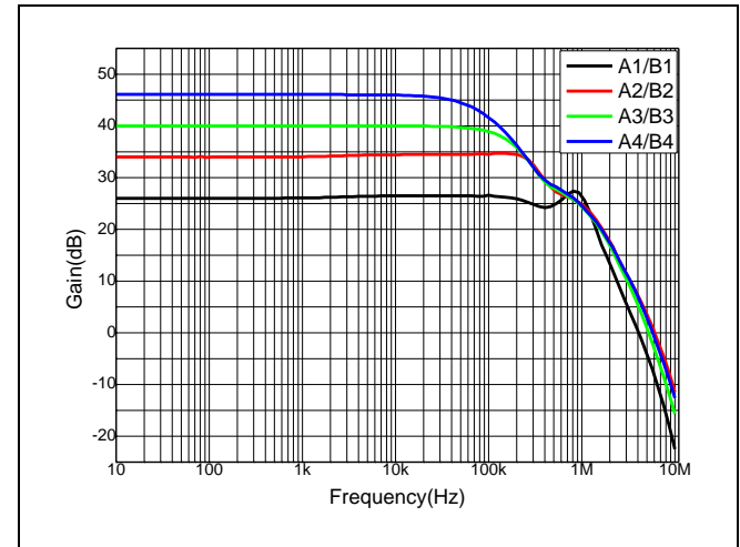
Figure 6. Gain vs. Frequency
