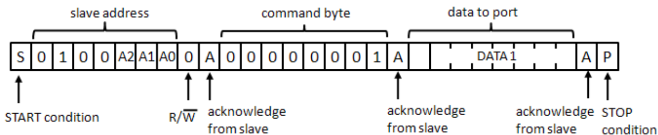
Figure 6: write to output register
