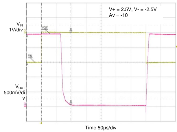
Positive Overvoltage Response
