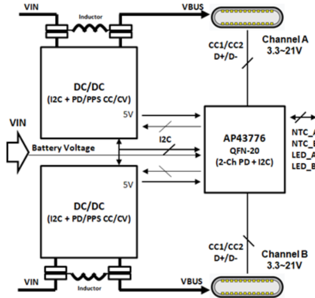
Figure 1. A two-channel car charger
