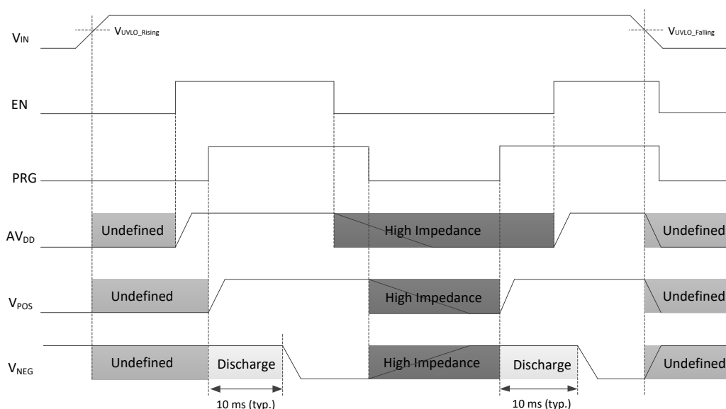
Figure 16. Startup and Shutdown Sequence Without Fast Discharge
