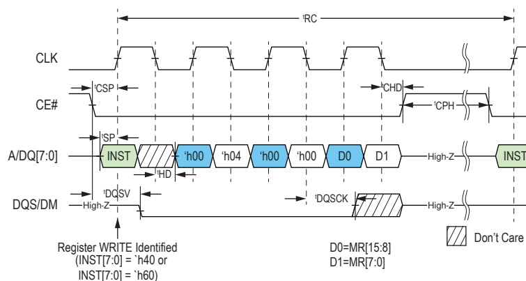
Figure 14: Register Write
