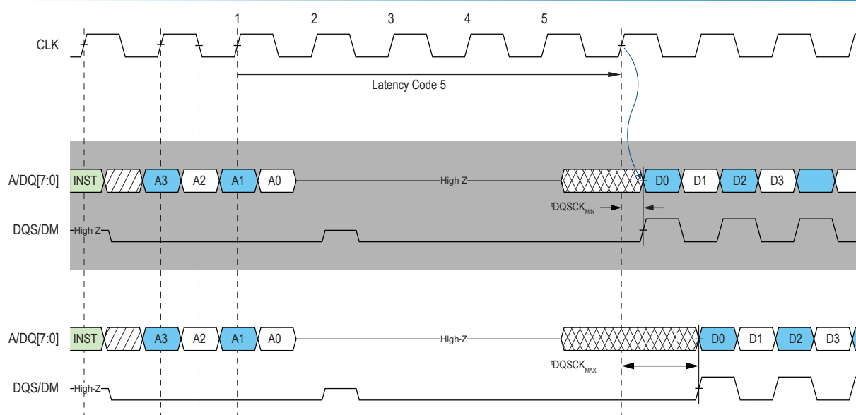
Figure 7: Read Latency & t_{DQSCK}
