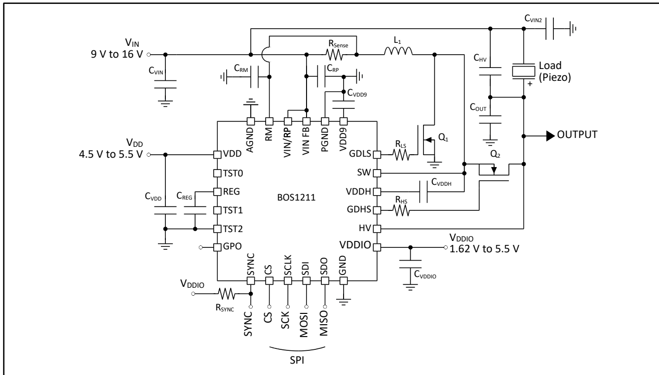
Figure 22: Typical schematic
