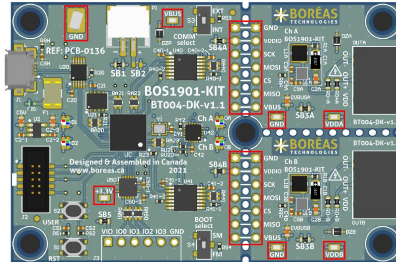
Figure 20: Probe hook location
