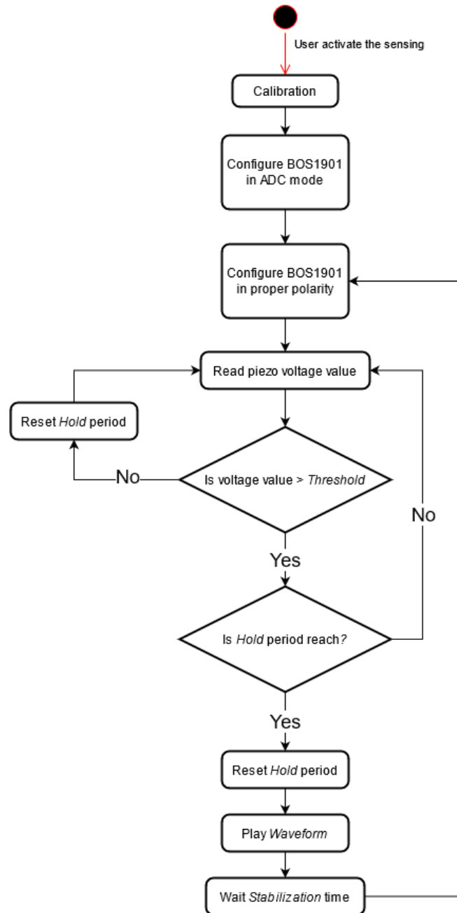
Figure 28: Sensing algorithm: flow chart.
