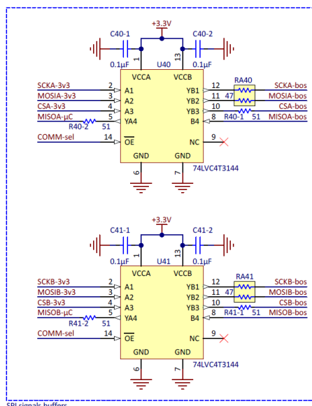
SPI signals buffers
