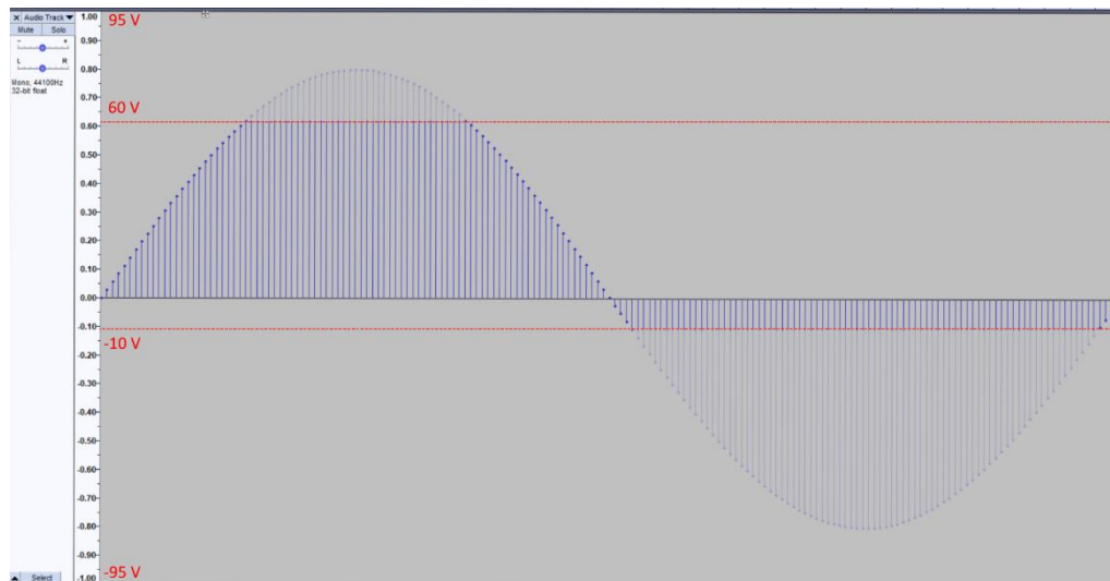
Figure 16:Audio signal with audio limiting
