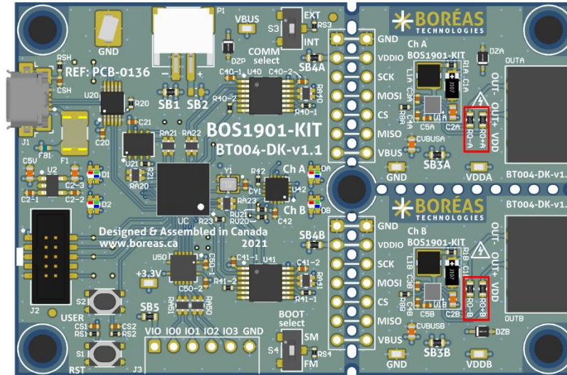
Figure 24: Low-pass filter resistors location
