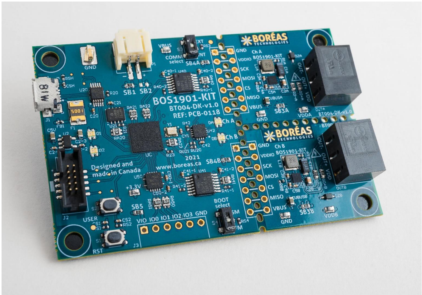
Figure 18: BOS1901-KIT PCB overview
