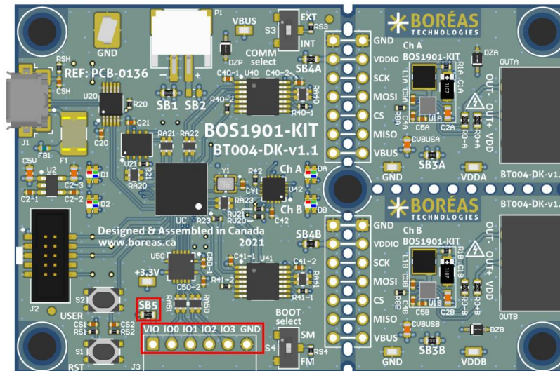
Figure 21: GPIOs and GPIOs supply voltage configuration solder bridge location
