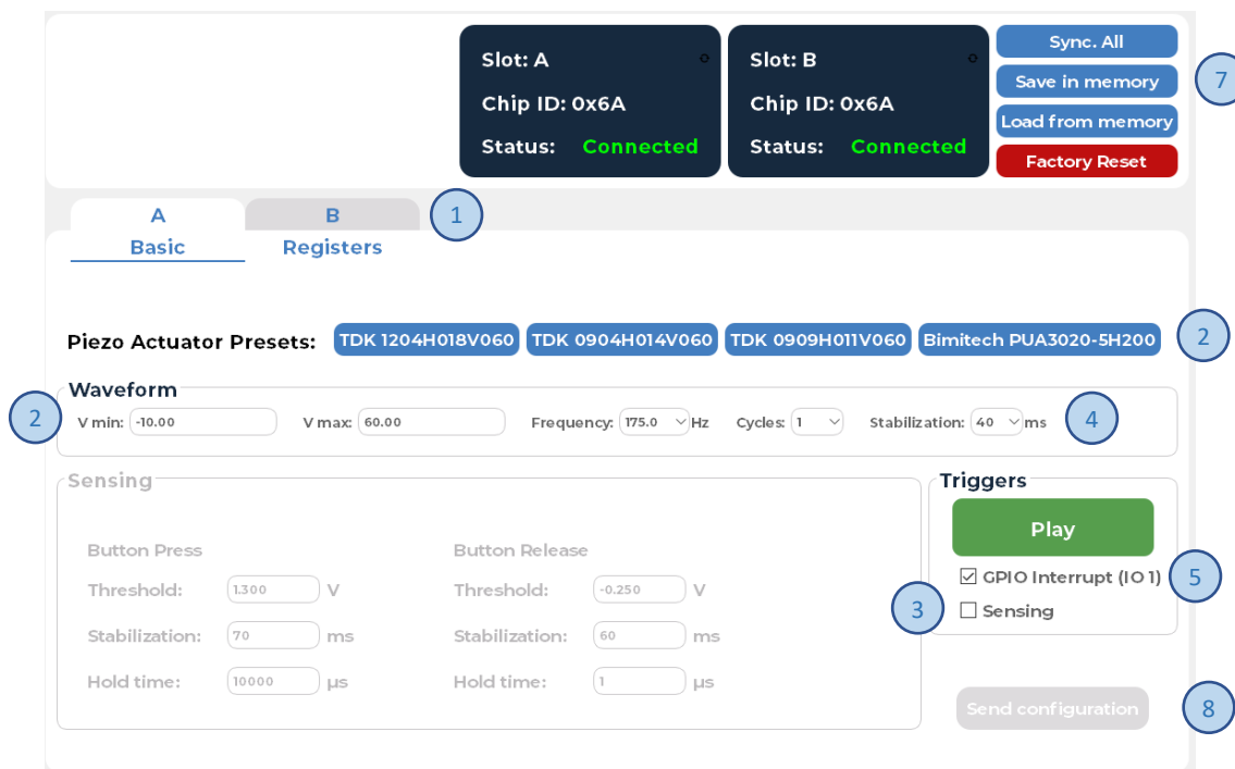
Figure 9: Play waveform – External trigger
