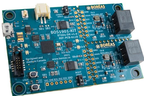
Figure 1: BOS1901-KIT overview
