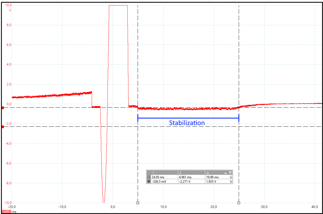
Figure 31: Sensing algorithm: stabilization
