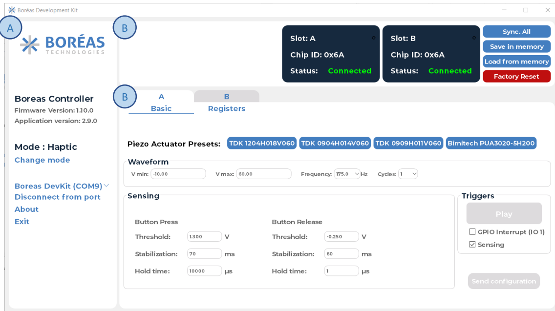
Figure 6 Application window when connected (Haptic mode)
