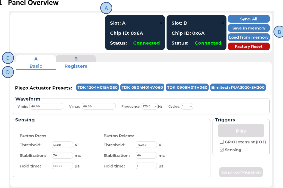
Figure 7: Panel overview – Haptic mode
