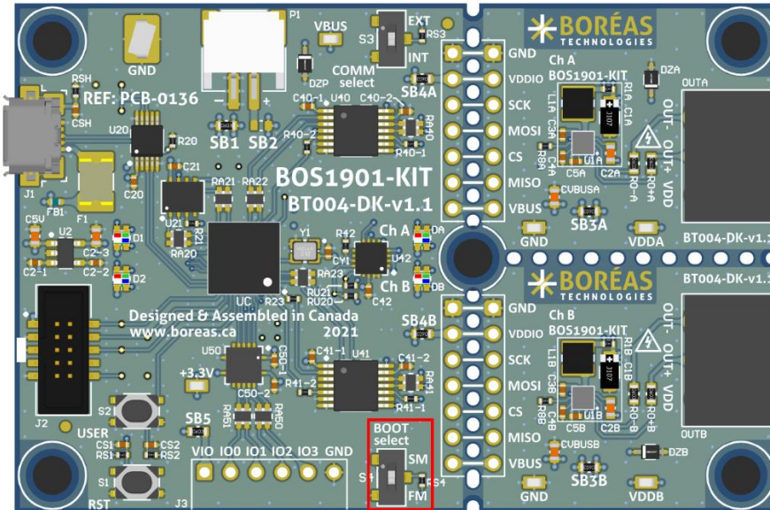
Figure 32 : Boot selection switch position
