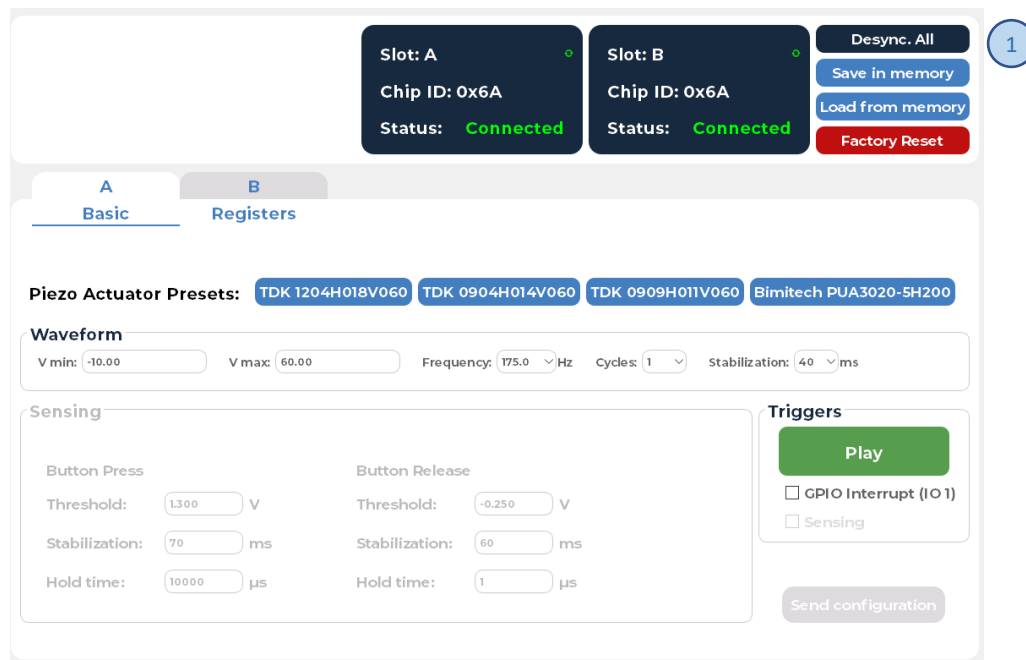
Figure 10: Play waveform – Sync mode
