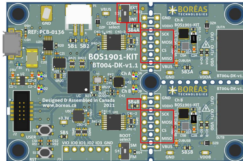
Figure 22: Comm selection switch and SPI header location
