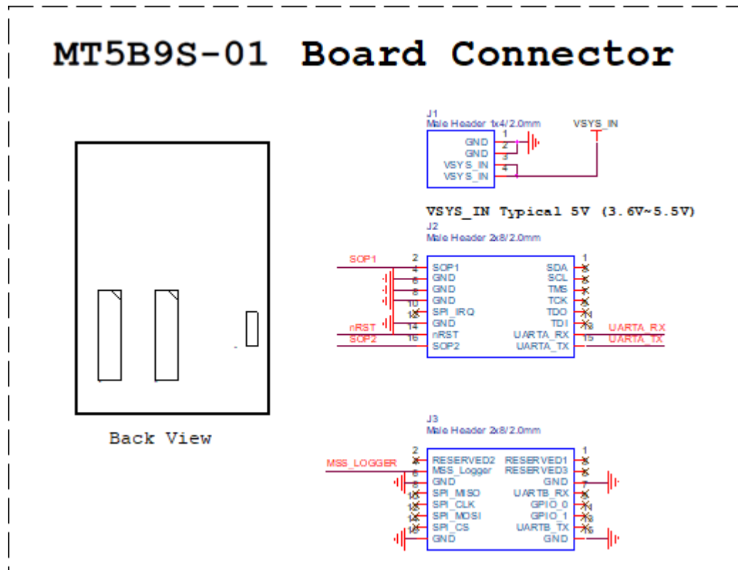
Figure 4-1. Board Connector of MT5B9S-01 device
