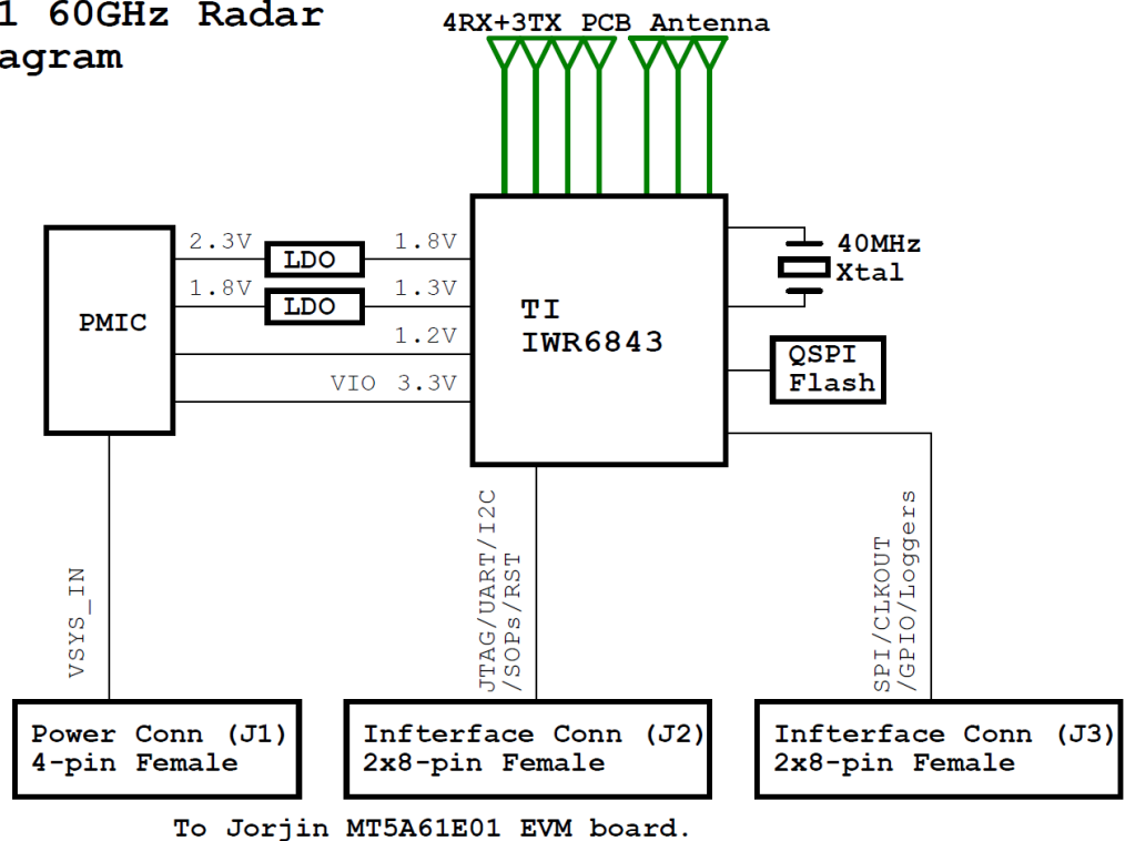
Figure 2-1. MT5B9S-01 Block Diagram
