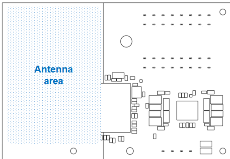
Figure 1-1. MT5B9S-01 Front View
