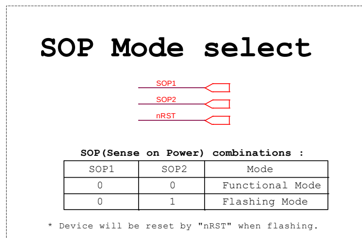
Figure 4-2. SOP mode of MT5B9S-01 device
