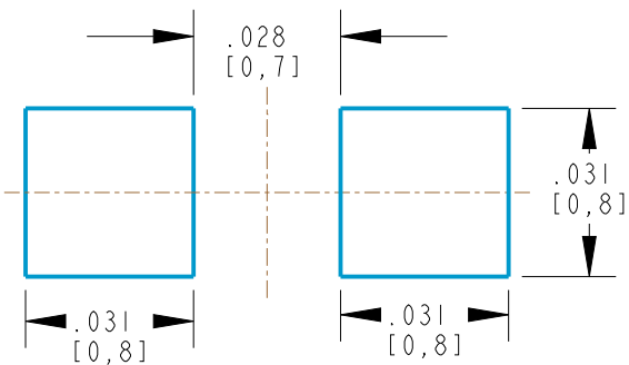
RECOMMEND PAD LAYOUT
