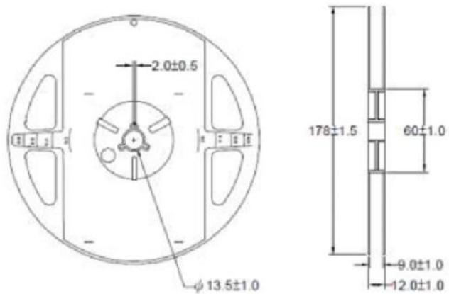
REEL DIMENSION (mm)
