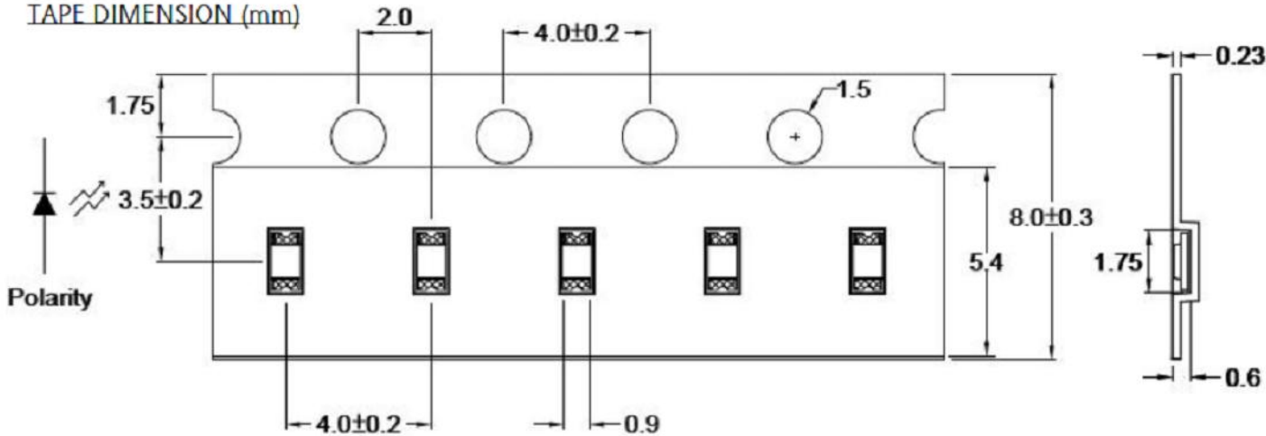
TAPE DIMENSION (mm)
