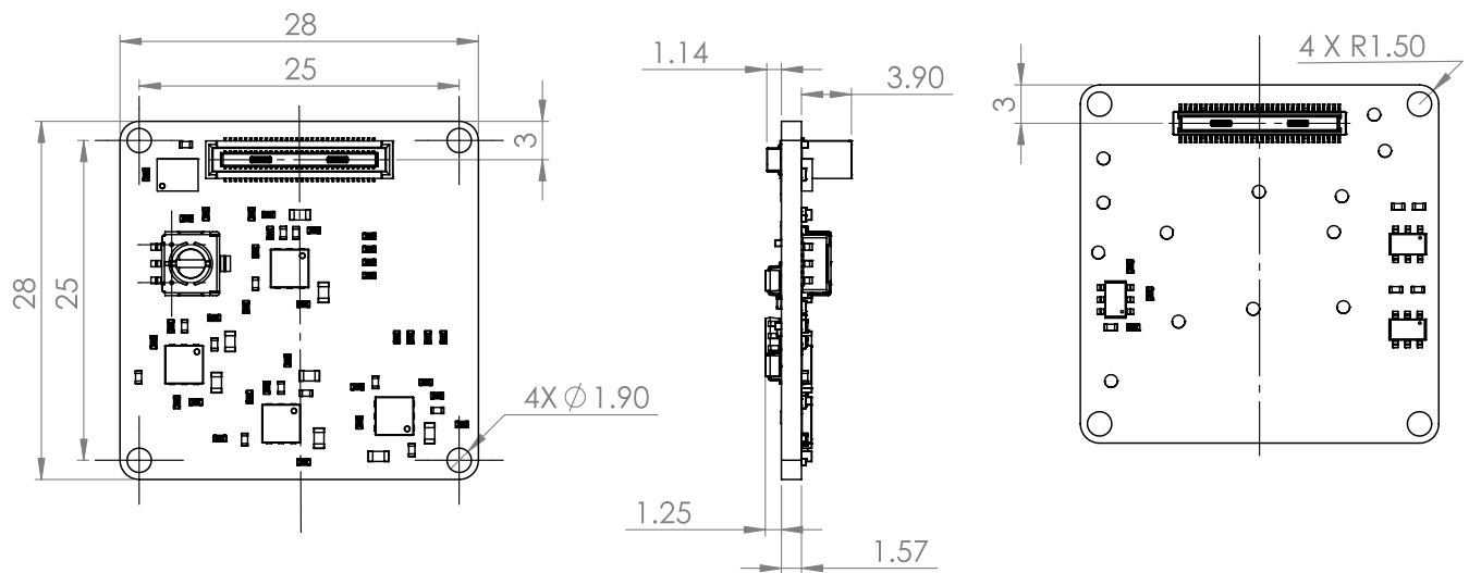
Figure 1: Technical Drawing of FSA-FTx/BC-V1
