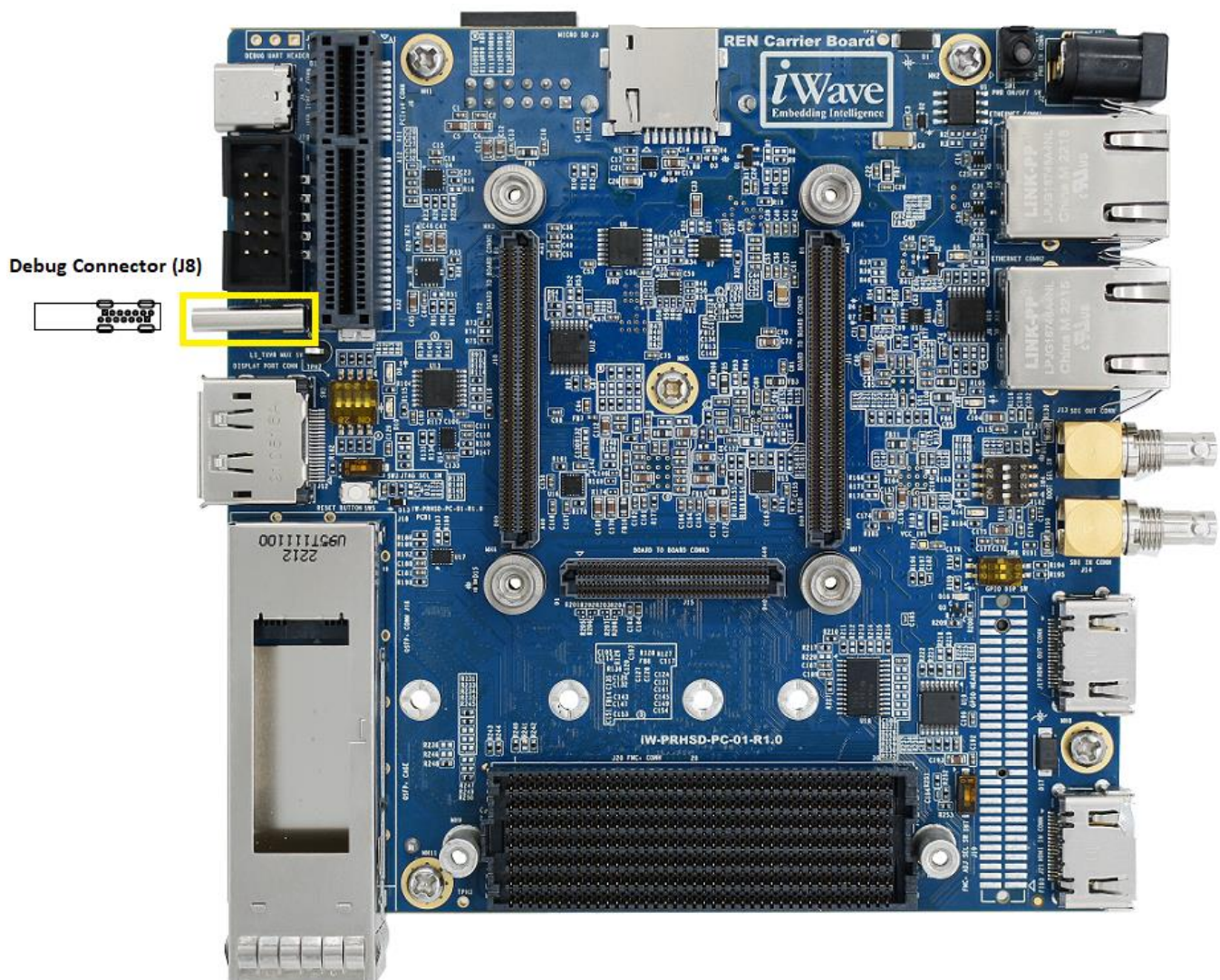
Figure 9: Debug Connector
