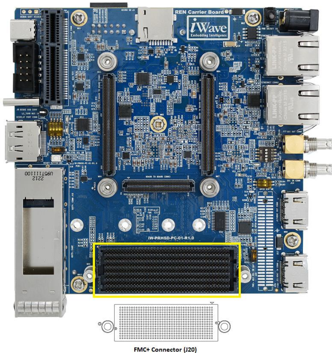
Figure 15: FMC+ Connector
