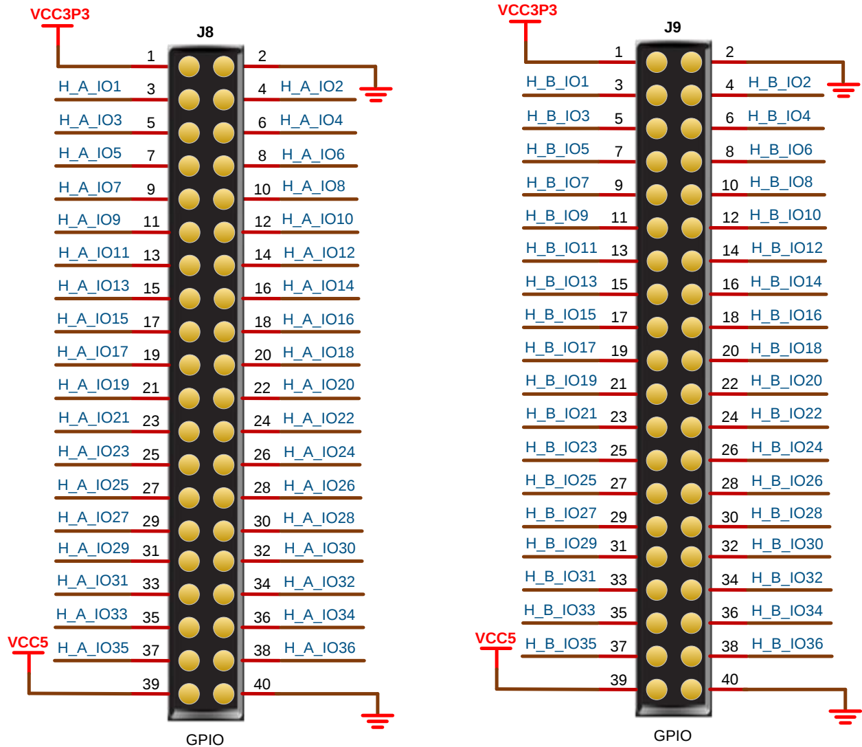
Figure 3-9 GPIO Circuit
