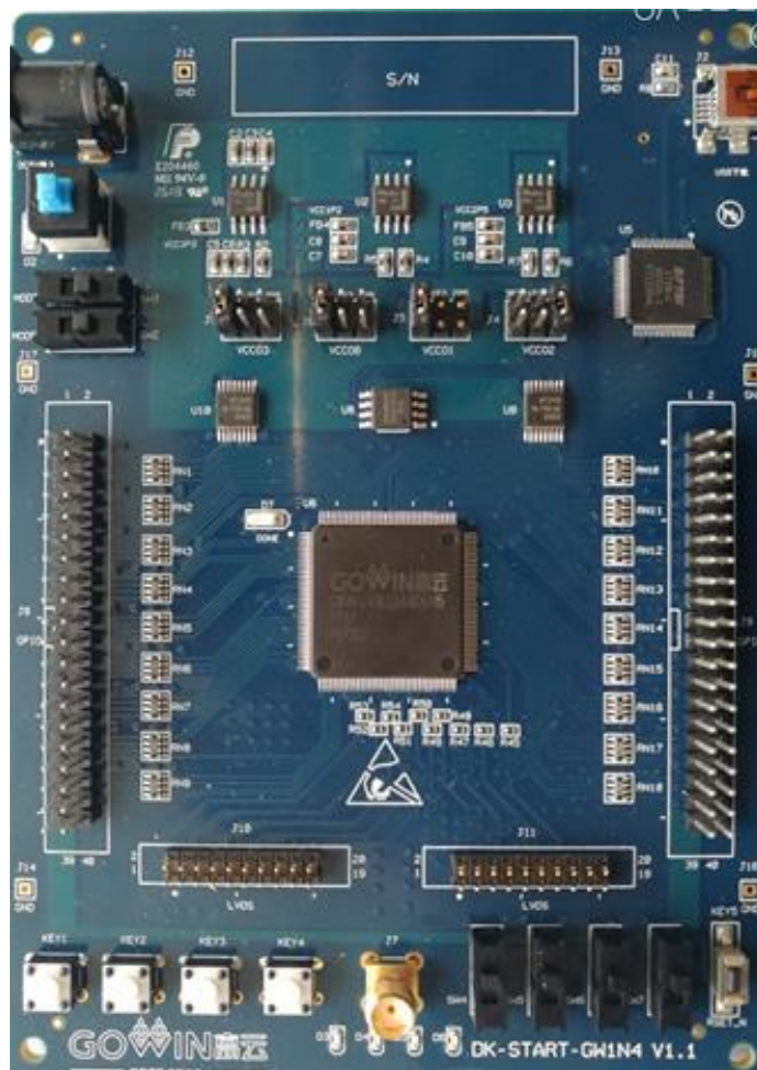
Figure 2-1 DK-START-GW1N V1.1
