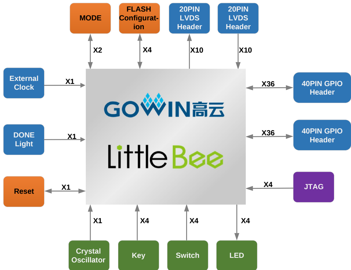
Figure 2-4 System Architecture
