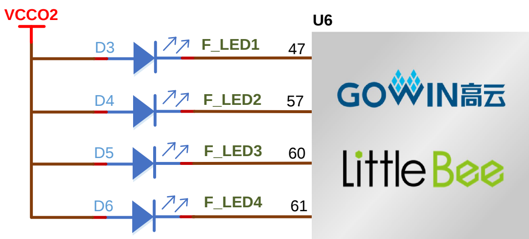
Figure 3-6 LED Circuit
