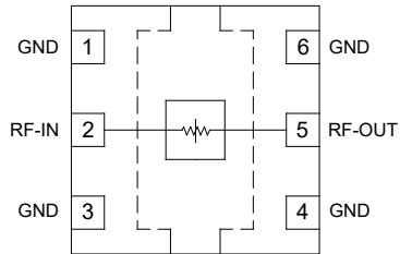
Figure 1. BAT-10+ Functional Diagram
