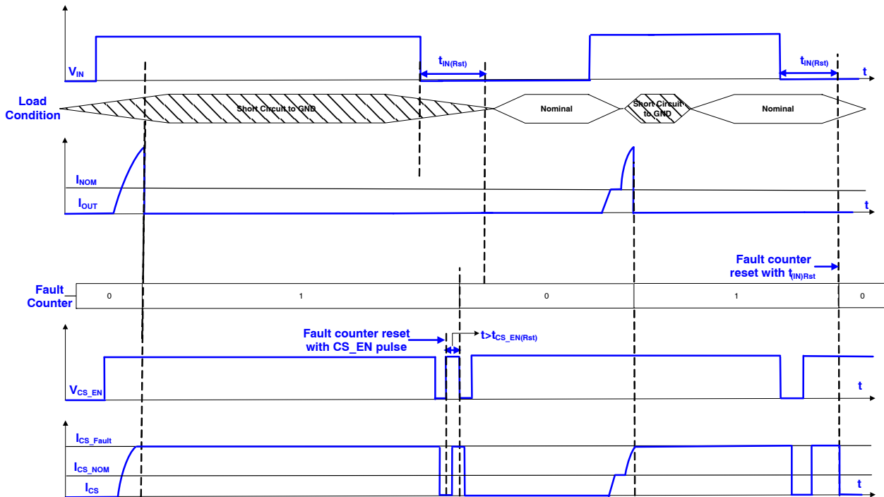
Figure 19. Retry Strategy in Case of Current Limit and/or Over-Temperature
