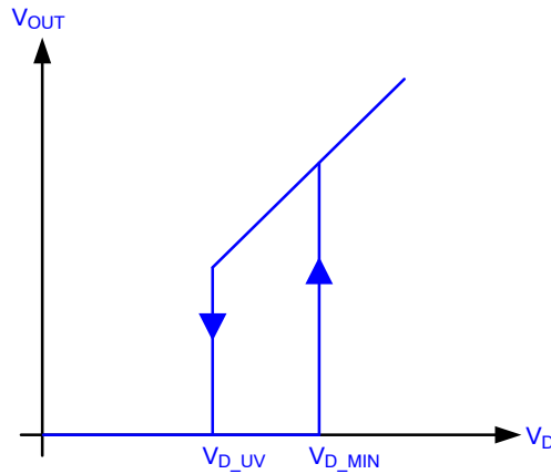
Figure 12. Under-voltage Behavior
