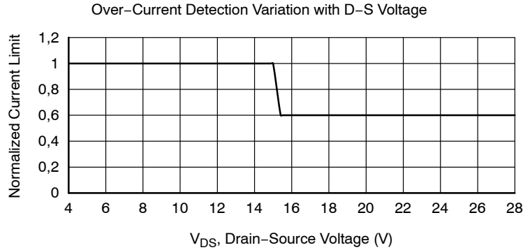
Figure 16. Over-Current Detection Variation with Drain-Source Voltage
