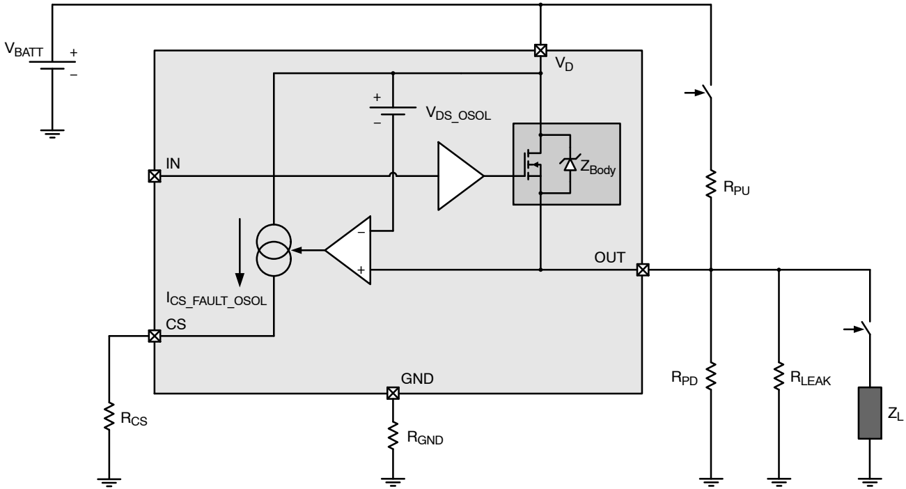
Figure 22. OFF State Open Load Detection Circuit
