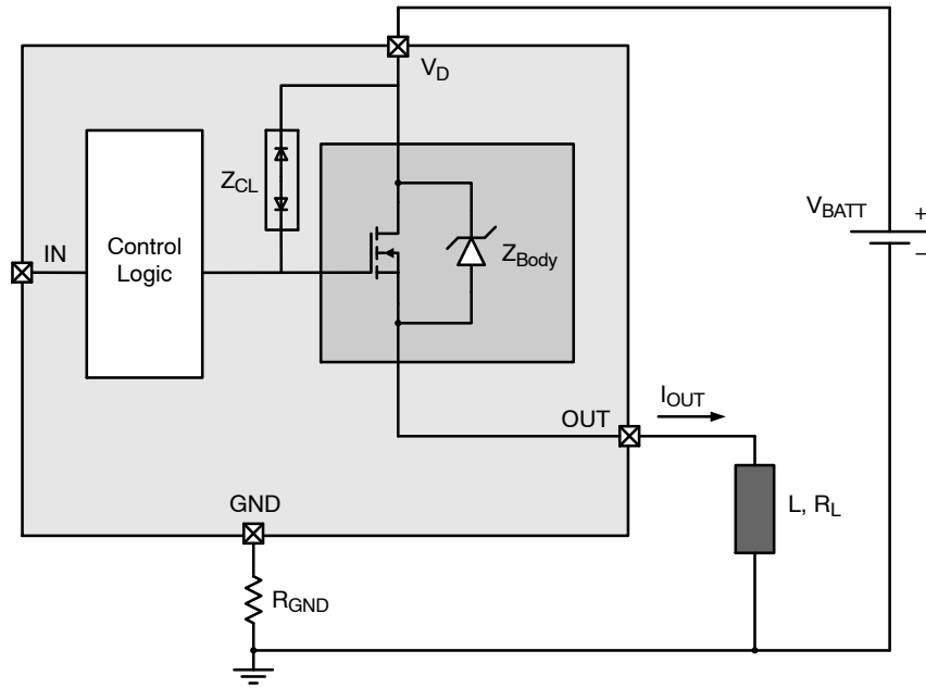
Figure 8. Output Clamping
