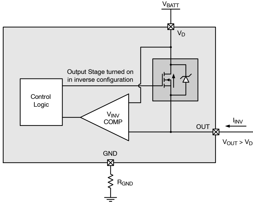
Figure 10. Inverse Current
