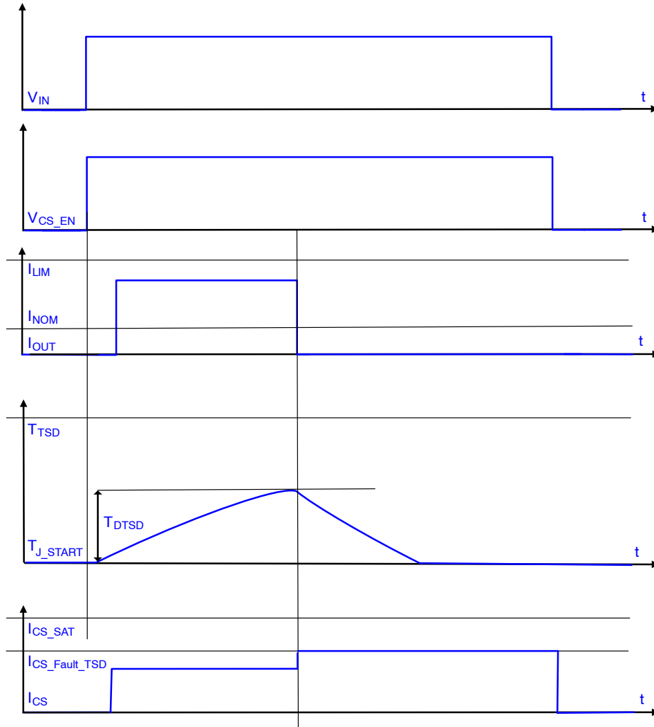
Figure 18. Over-Temperature Protection
