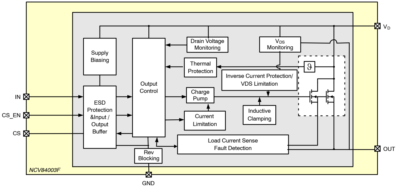
Figure 1. Block Diagram
