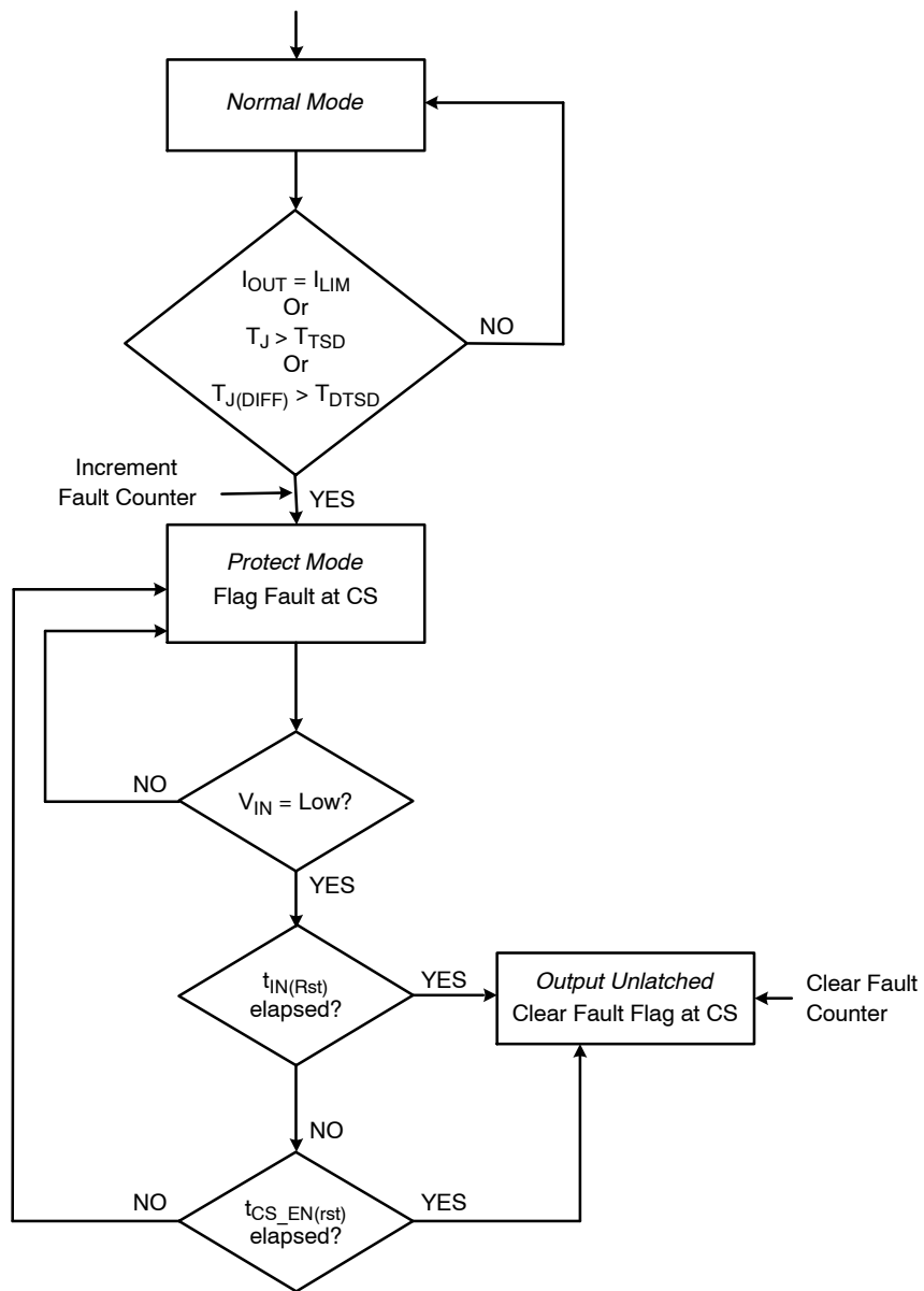
Figure 20. On-State Re-try Strategy Flowchart
