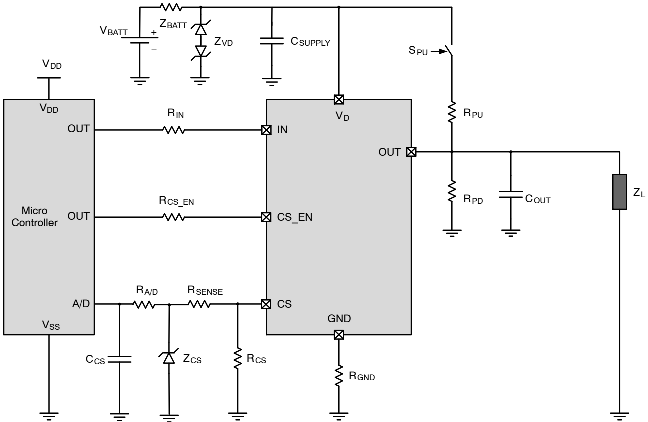
Figure 4. Application Diagram
