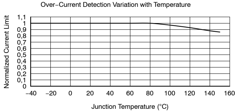
Figure 17. Over-Current Detection Variation with Junction Temperature
