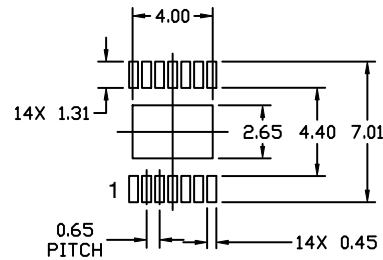
RECOMMENDED MOUNTING FOOTPRINT
