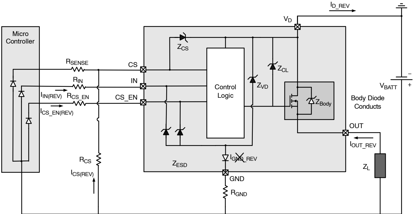
Figure 15. Reverse Battery Protection Circuit
