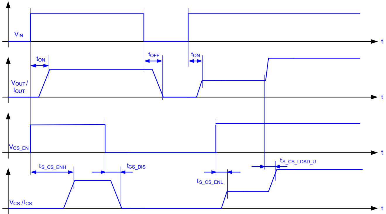
Figure 21. Current Sense Timings
