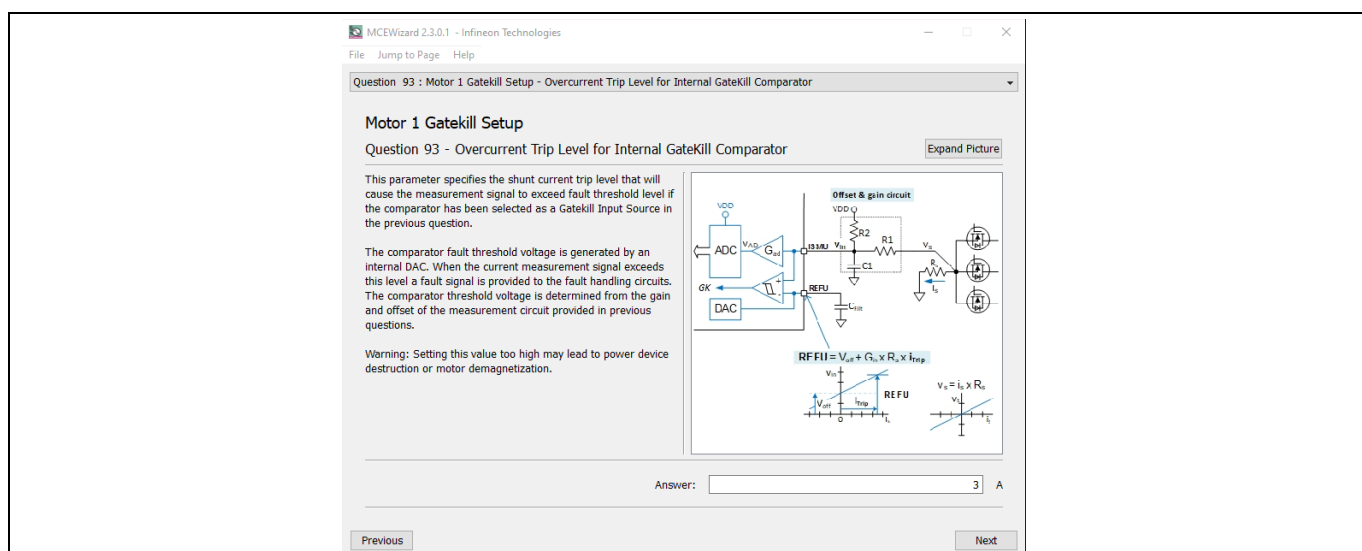
Figure 14 Over current trip level setting in MCEWziard
