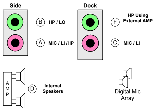
Figure 10. Port Configurations
