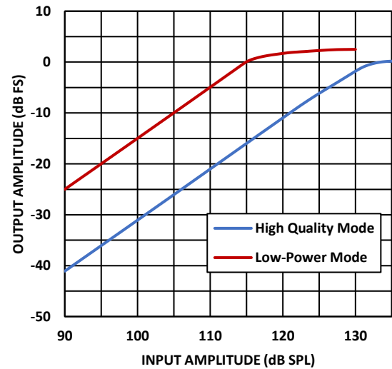
Figure 7. Linearity
