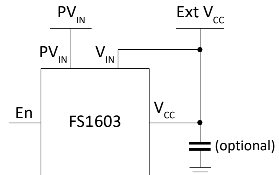
Figure 7 Using an external bias voltage
