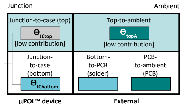
Figure 18 Thermal resistances of the FS1603
