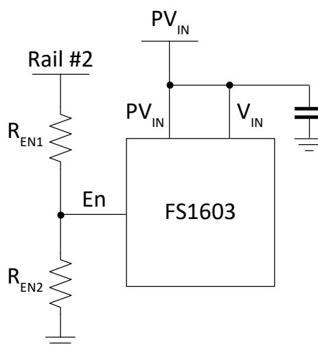
Figure 9 En pin used to monitor other rails for sequencing purposes
