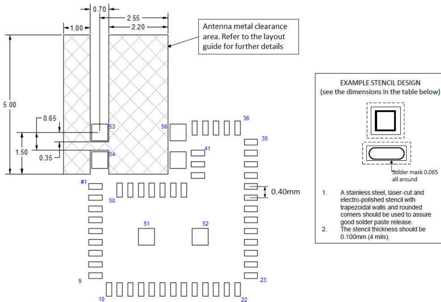
Figure 8.3. BGM11S recommended land pattern
