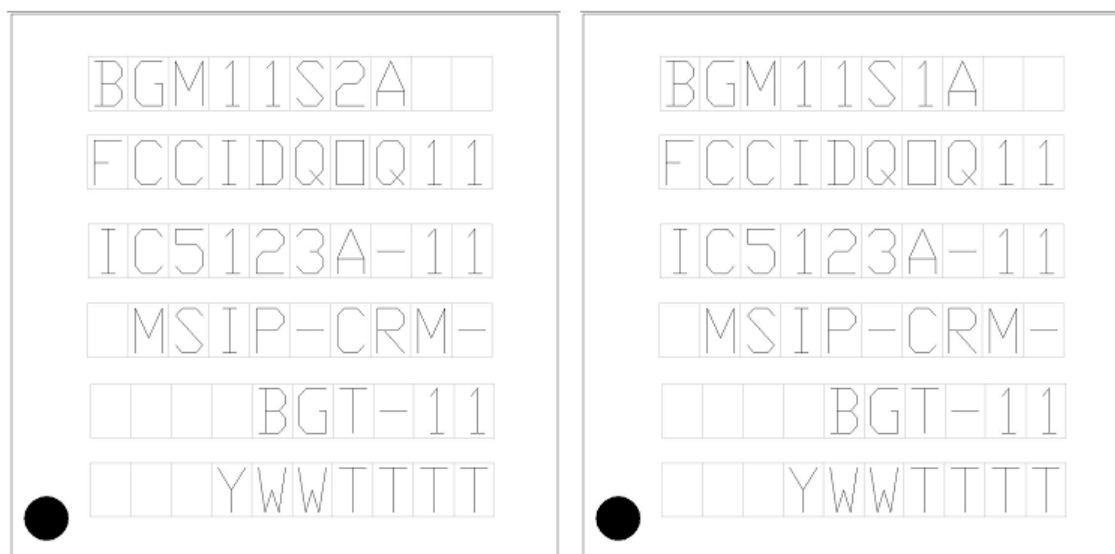
Figure 8.2. BGM11S Package Marking
