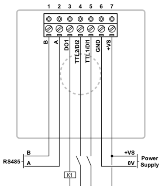
CONNECTION EXAMPLE
