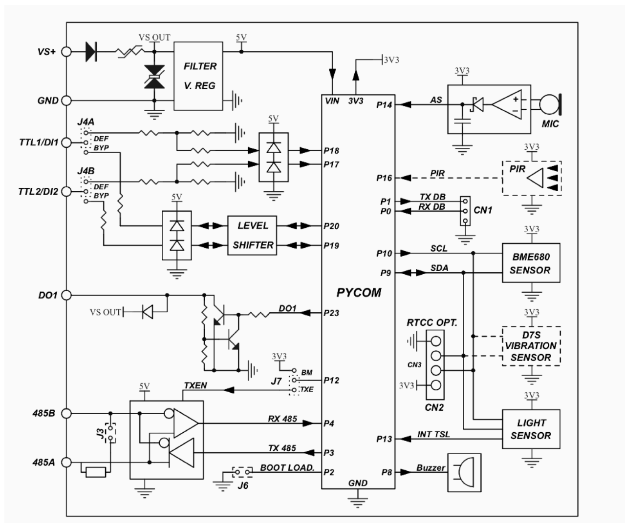
BLOCK DIAGRAM
