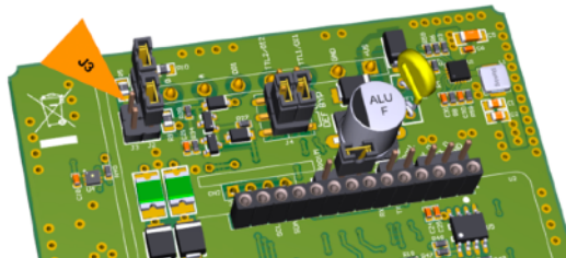
RS-485 JUMPERS POSITION
