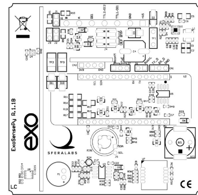
BOARD LAYOUT (TOP VIEW)
