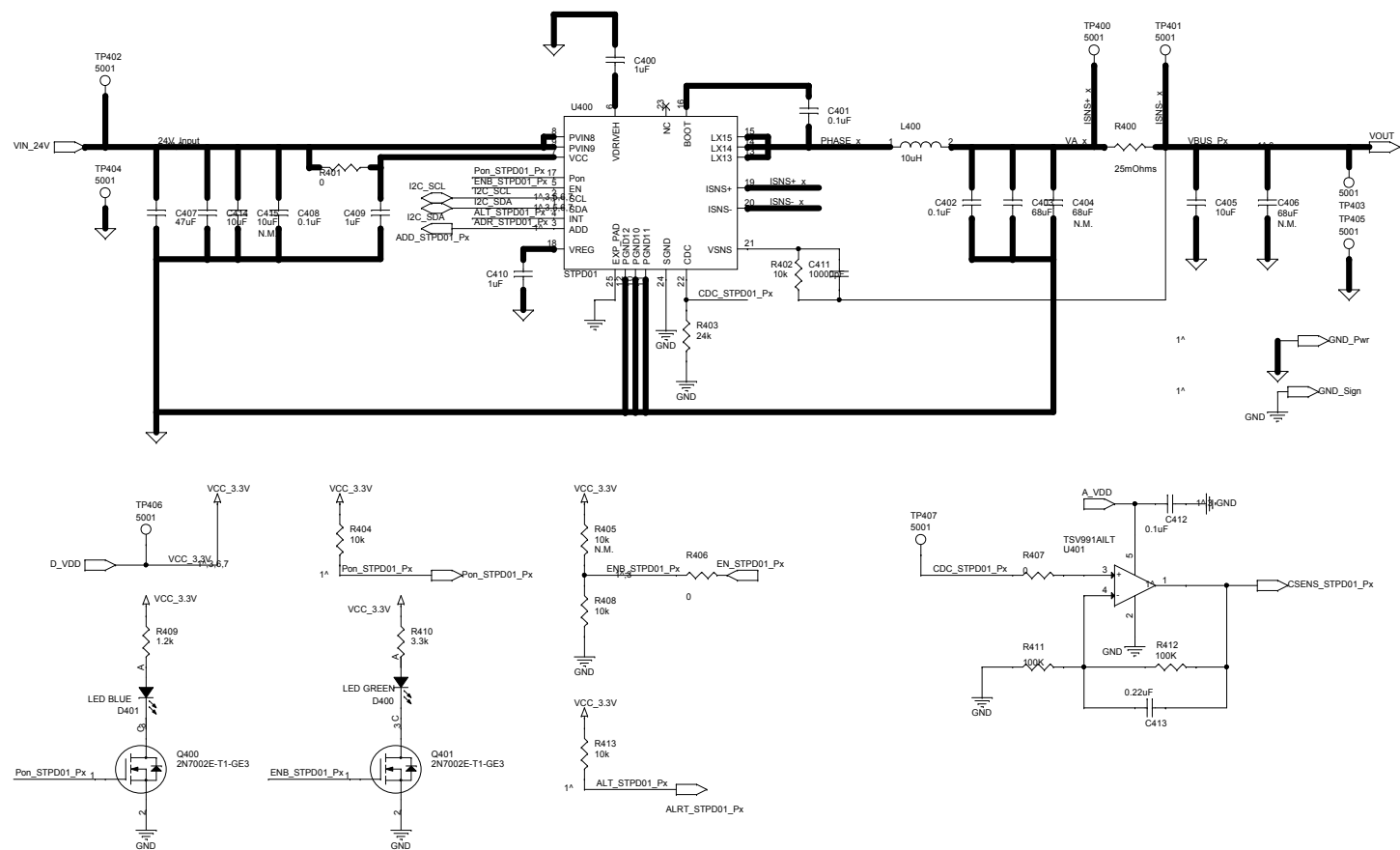
Figure 4. STEVAL-2STPD01 circuit schematic (4 of 7)
