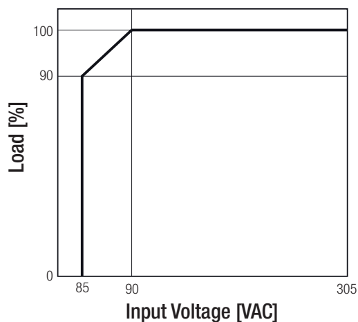
Line Derating (3)
