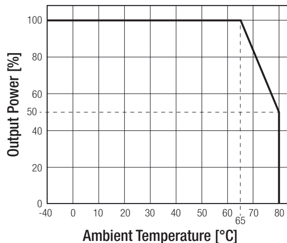
Derating Graph
