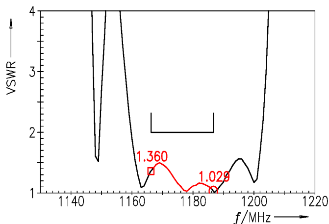
Figure 5: Reflection coefficient at input port.
