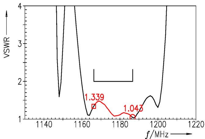
Figure 6: Reflection coefficient at output port.
