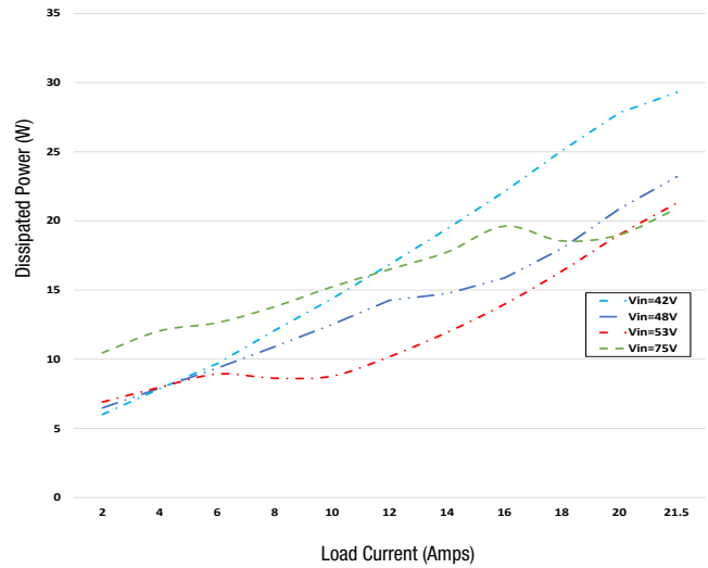
Dissipated Power vs. Load Current & Input Voltage @ 25°C
