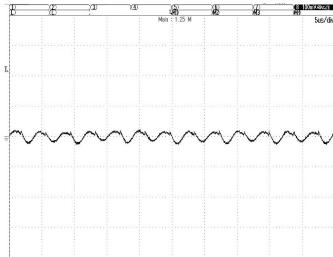
Output Ripple & Noise (48Vin)
