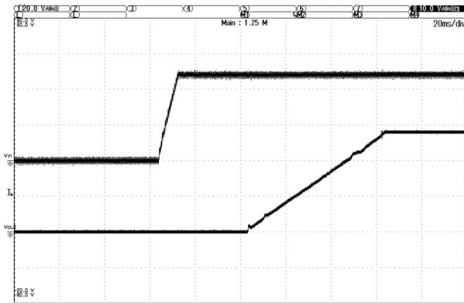
Start-up Voltage (48Vin)
