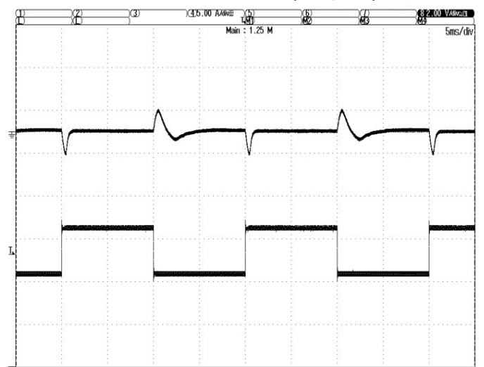
Load Transient Waveform (1A/uS, 48Vin)
