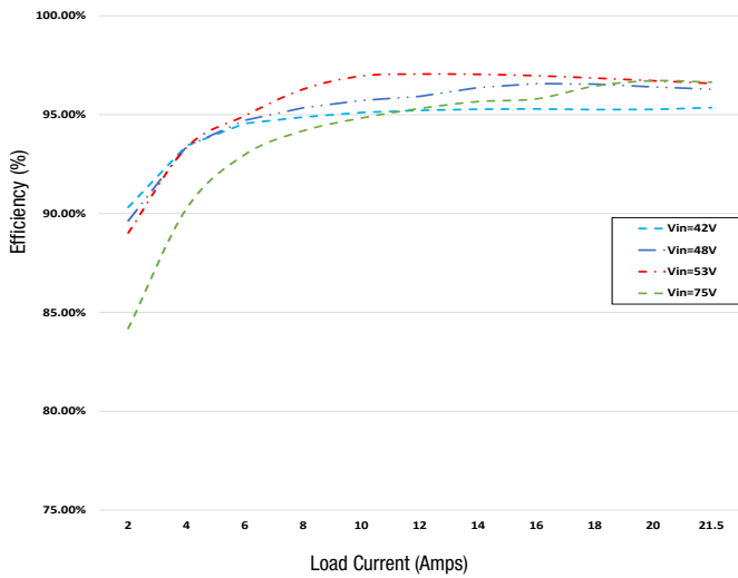
Efficiency vs. Load Current & Input Voltage @ 25°C
