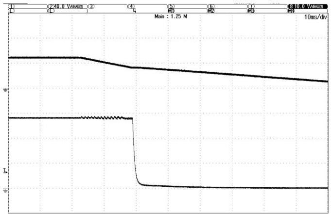
Shut-down Voltage (48Vin)
