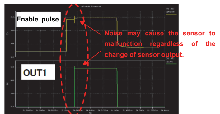
<Enable pulse waveform noise and malfunction of OUT1>
