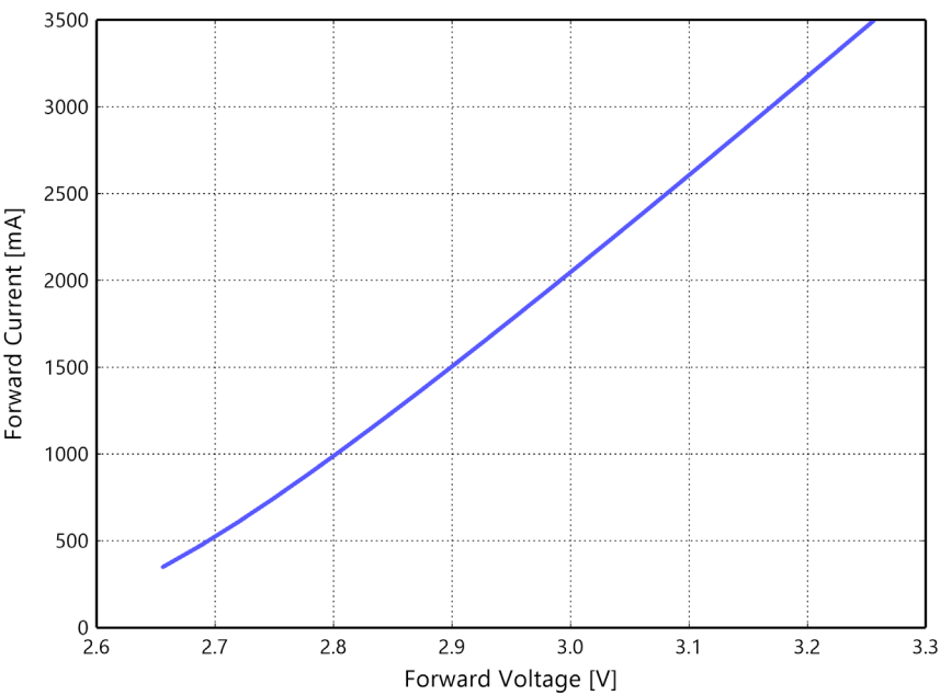
Figure 4. Typical forward current vs. forward voltage for LUXEON HL4Z at T j =85°C.
