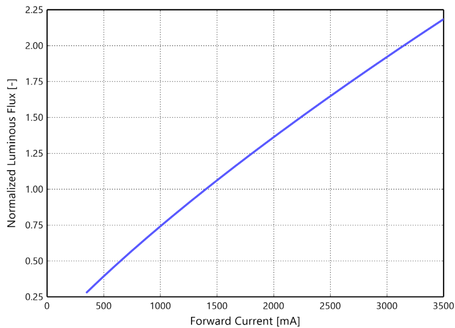
Figure 3. Typical normalized light output vs. forward current for LUXEON HL4Z at 1400mA, T j =85°C.
