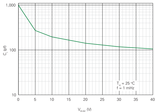
Fig. 4. Junction Capacitance vs. Reverse Voltage
