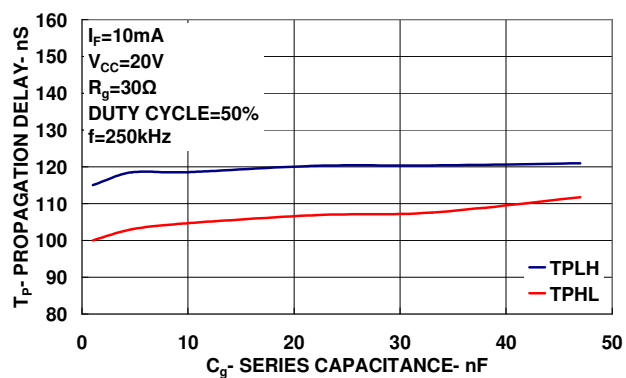
Figure 13 : Propagation vs. Load Capacitance
