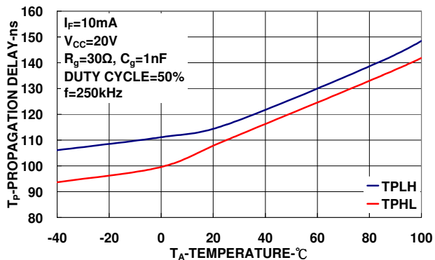
Figure 11 : Propagation vs. Temperature
