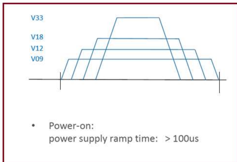
Figure 7 - BNU domain power supply ramp time requirement
