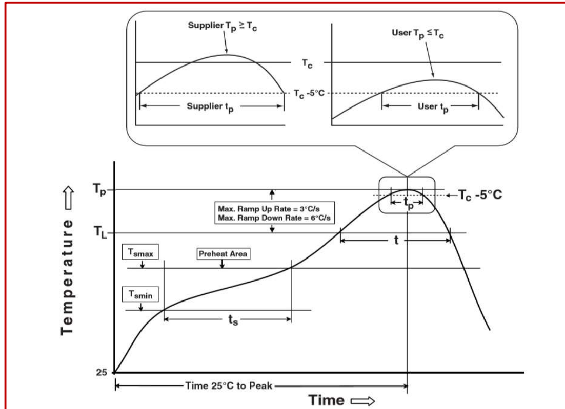
Figure 13 - Reflow profile
