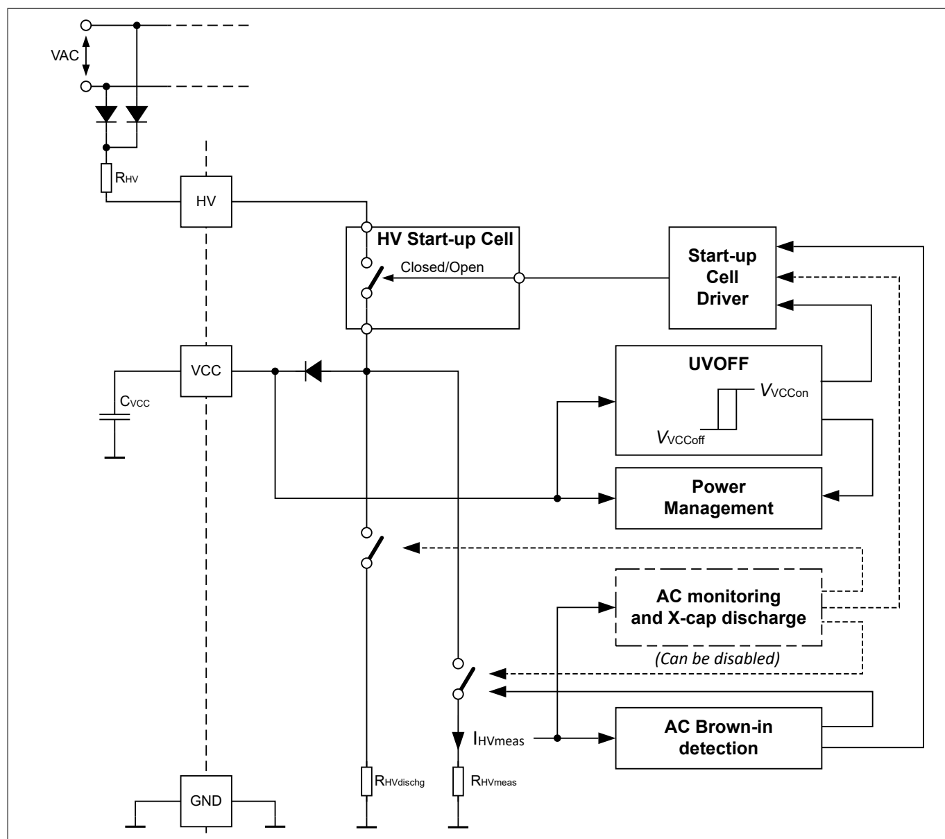
Figure 5 HV control for start-up, brown-in detection and X-capacitor discharge
