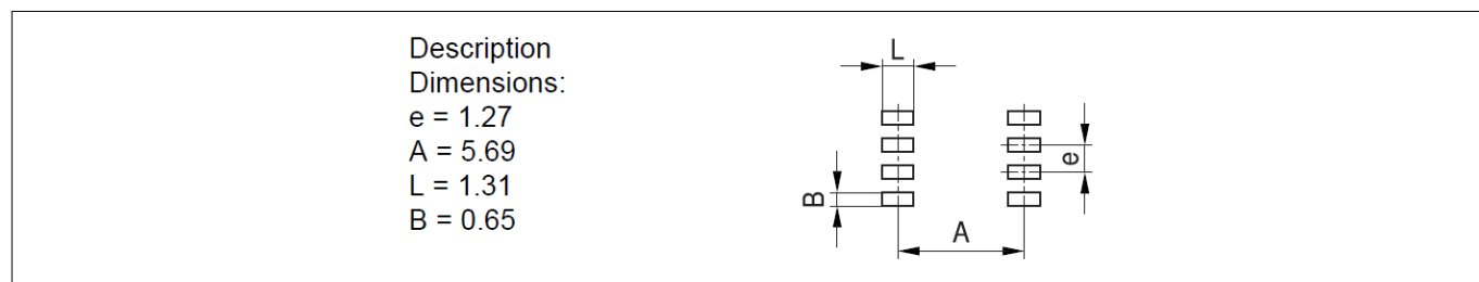
Figure 28 PG-DSO-14 footprint
