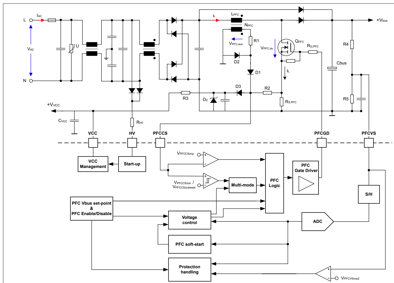
Figure 8 QRM-PFC circuit arrangement and associated PFC control
