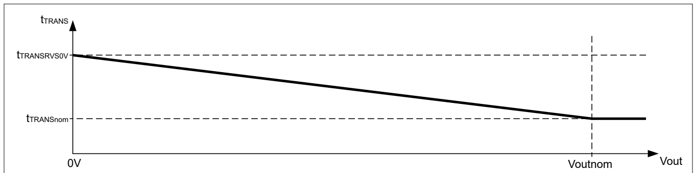
Figure 17 V_{out} compensation for t_{TRANS} in ZV-RVS mode
