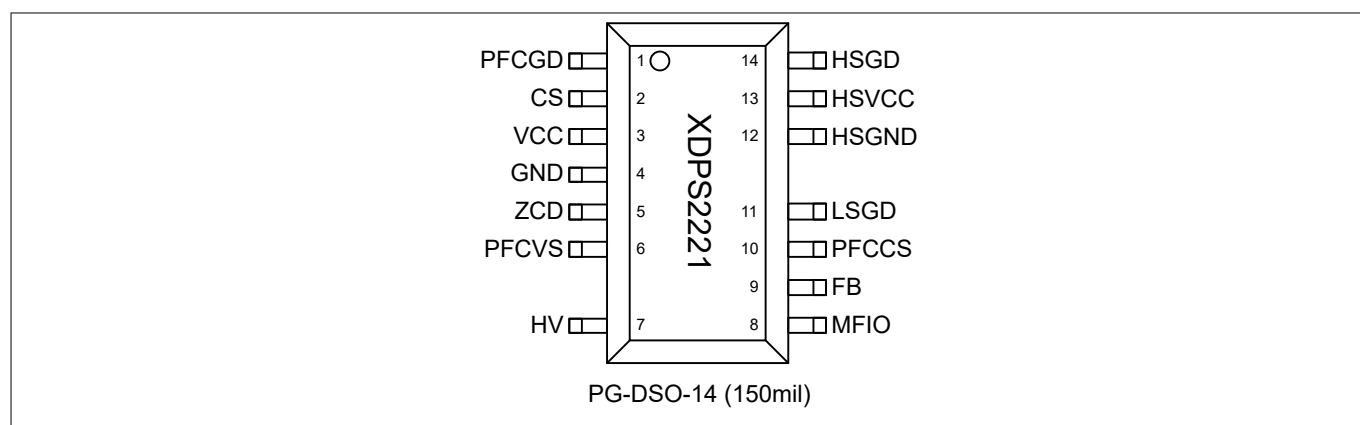
Figure 1 Pin configuration
