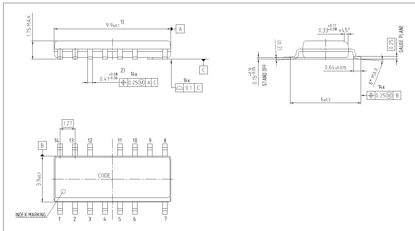
Figure 27 PG-DSO-14 outline
