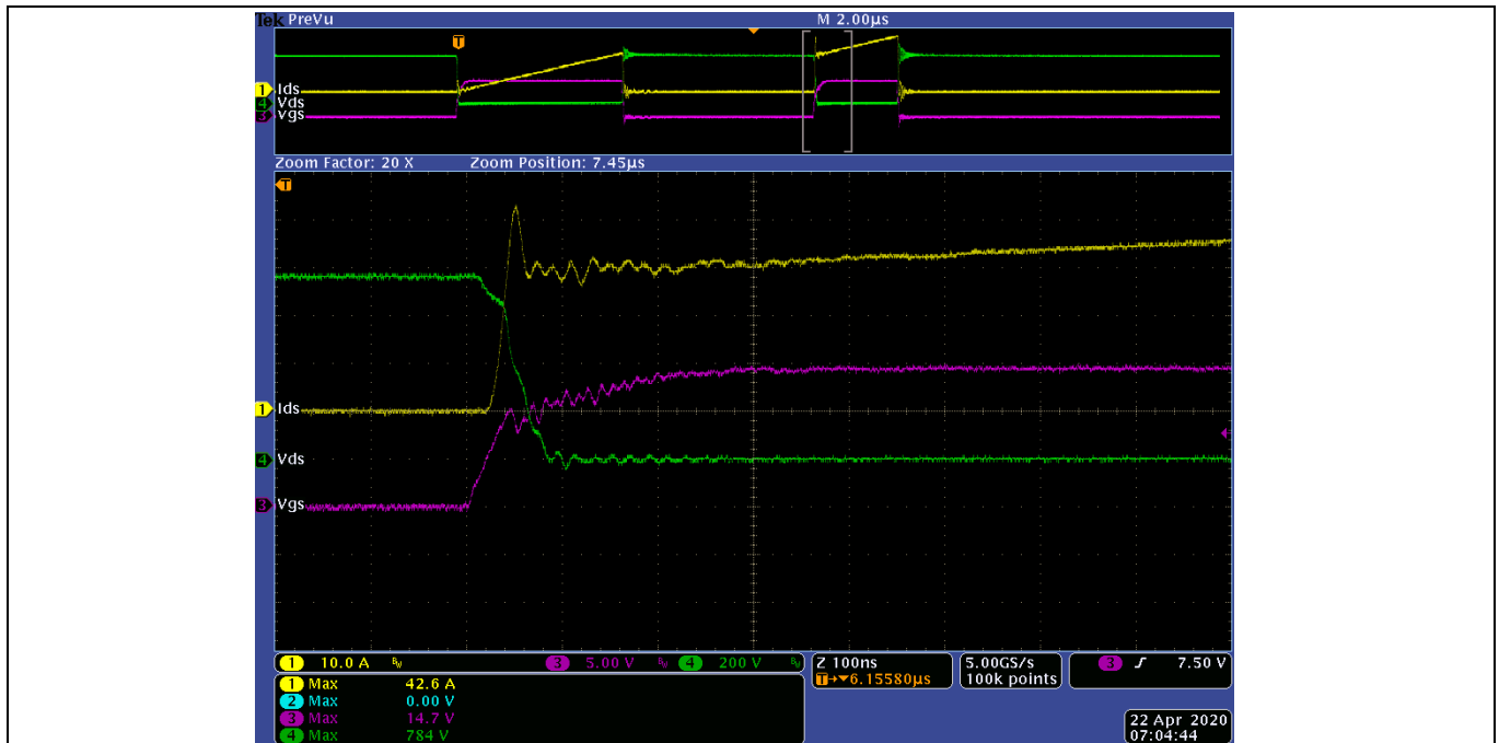
Figure 7 Turn-on of the REF_SiC_D2Pak_MC_V0.1
