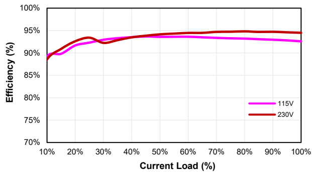
CFM600S280 (Eff Vs Io)
