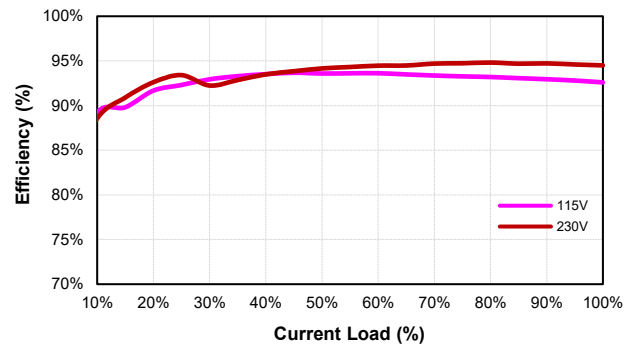
CFM600S300 (Eff Vs Io)
