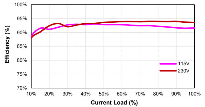
CFM600S150 (Eff Vs Io)
