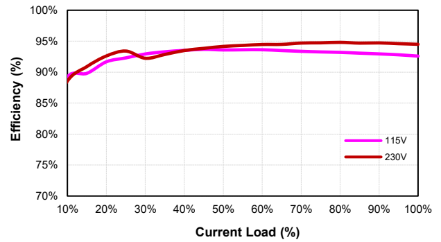
CFM600S240 (Eff Vs Io)
