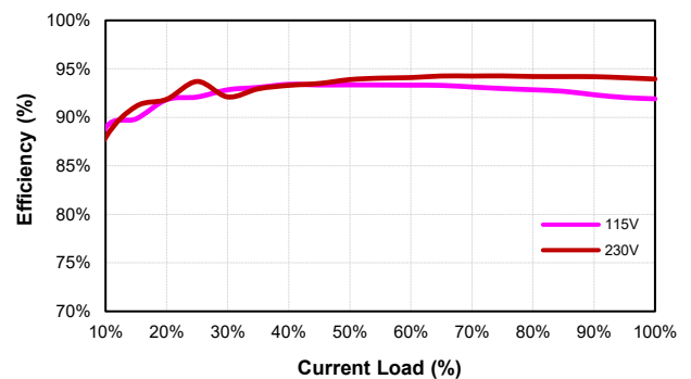
CFM600S480 (Eff Vs Io)
