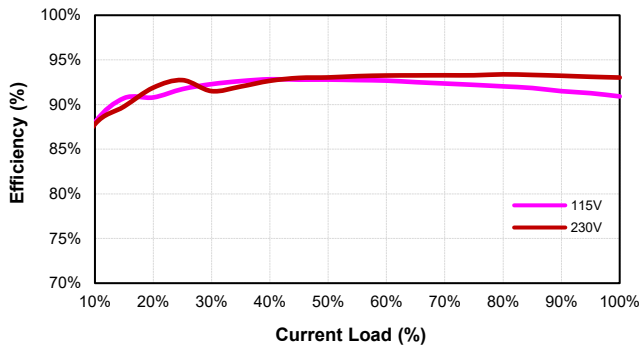
CFM600S120 (Eff Vs Io)
