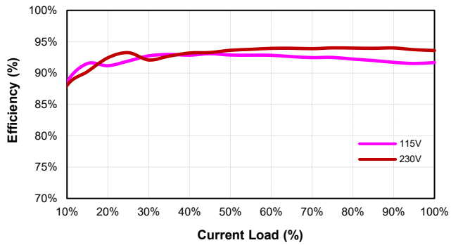
CFM600S180 (Eff Vs Io)
