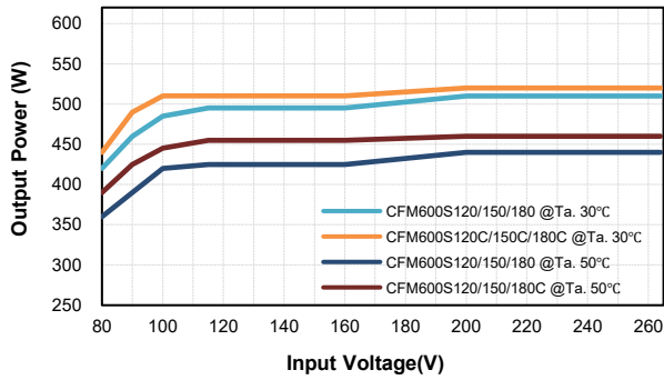
Output Power Vs Input Voltage
