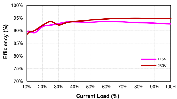
CFM600S360 (Eff Vs Io)
