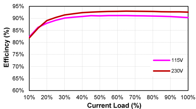
TR220M480 (Eff Vs Io)
