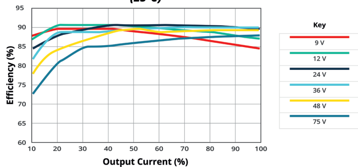
EFFICIENCY VS OUTPUT LOAD PRQE75W-E12-S12-D (25°C)
