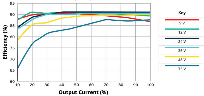
EFFICIENCY VS OUTPUT LOAD PRQE75W-E12-S24-D (25°C)
