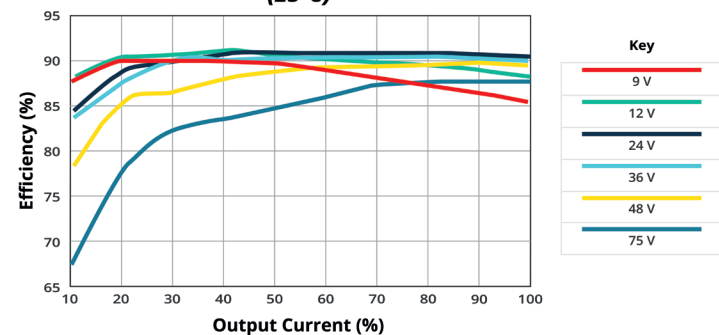
EFFICIENCY VS OUTPUT LOAD PRQE75W-E12-S15-D (25°C)
