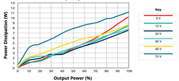
POWER DISSIPATION VS OUTPUT POWER PRQE75W-E12-S48-D (25°C)
