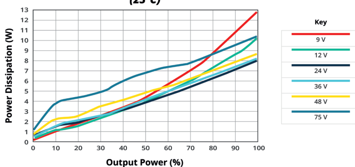
POWER DISSIPATION VS OUTPUT POWER PRQE75W-E12-S15-D (25°C)
