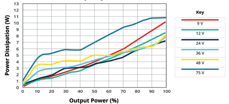
POWER DISSIPATION VS OUTPUT POWER PRQE75W-E12-S48-D (25°C)
