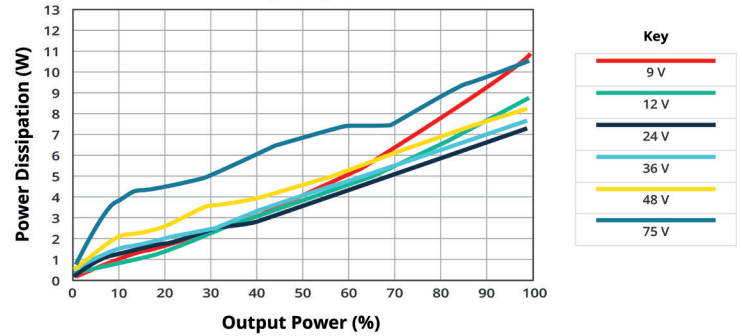
POWER DISSIPATION VS OUTPUT POWER PRQE75W-E12-S24-D (25°C)
