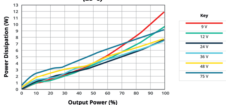
POWER DISSIPATION VS OUTPUT POWER PRQE75W-E12-S12-D (25°C)
