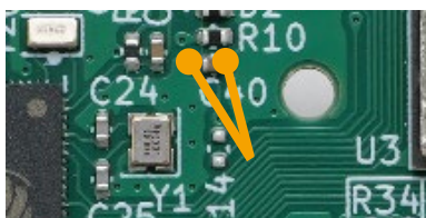
Fig. 5.2.1. Turning ESP32-P4 into download mode
