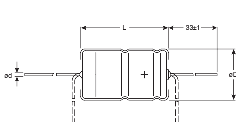
Form AA: Axial in box (bulk) Case \phi D \times L = 10 \times 30 to 21 \times 38 \text{mm}
