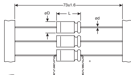
Form BA: Taped in box (ammopak), case \phi D \times L = 6.5 \times 18 to 10 \times 25 \text{mm}
