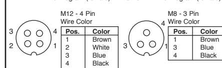
M12 - 4 Pin Wire Diagram (female) M8 - 3 Pin Wire Diagram (female)
