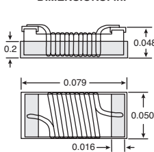
DIMENSIONS: in.
