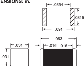
DIMENSIONS: in.
