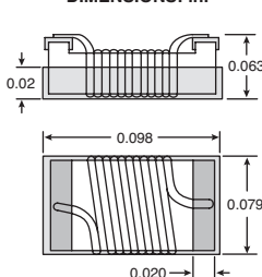
DIMENSIONS: in.
