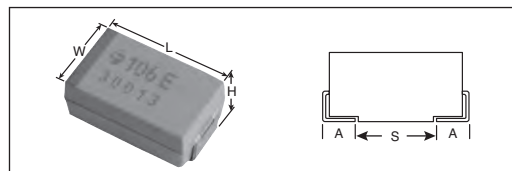
DIMENSIONS: mm (in.)
