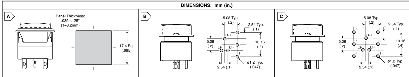
DIMENSIONS: mm (in.)
